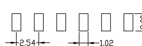
PCB LAYOUT
